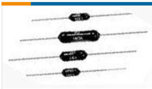
TE 零件编号9-1879664-1 H8 10K 0.1% 15PPM
